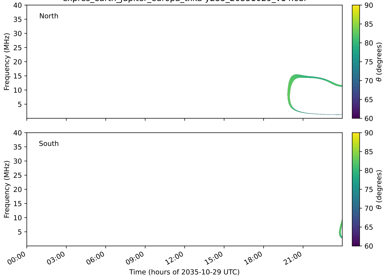
expres_earth_jupiter_europa_txka-y235_20351029_v14.cdf
