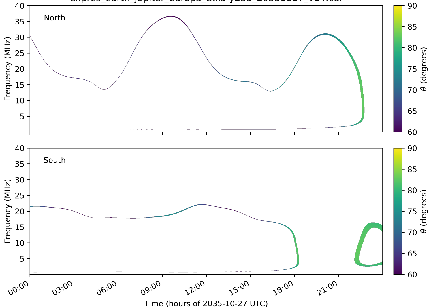
expres_earth_jupiter_europa_txka-y235_20351027_v14.cdf
