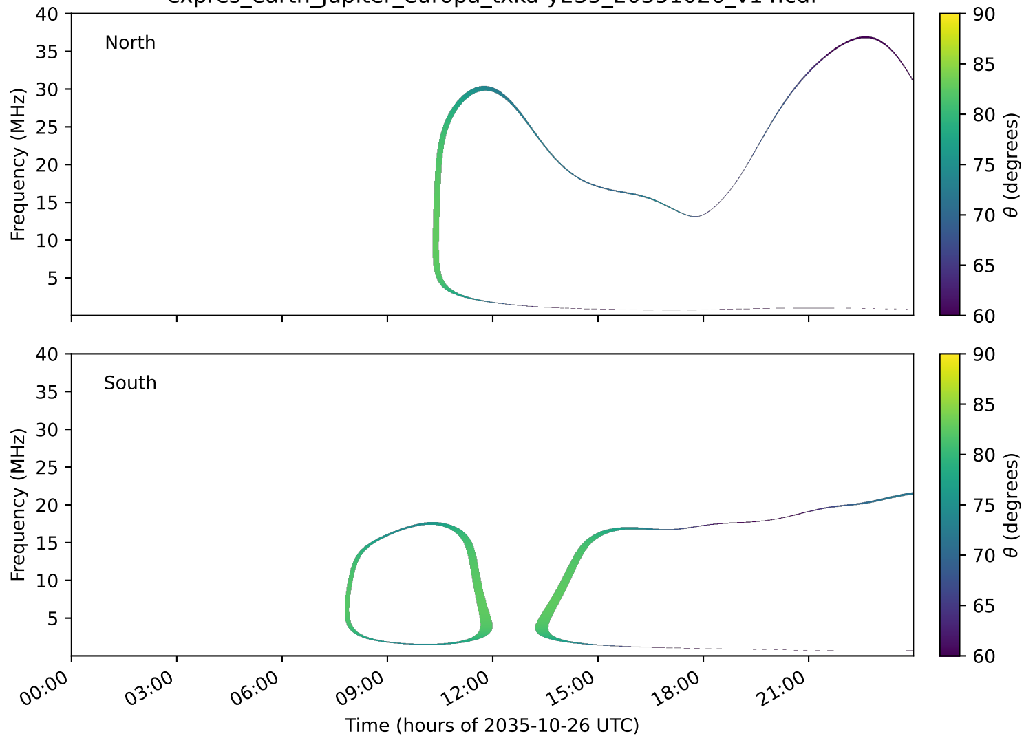
expres_earth_jupiter_europa_txka-y235_20351026_v14.cdf
