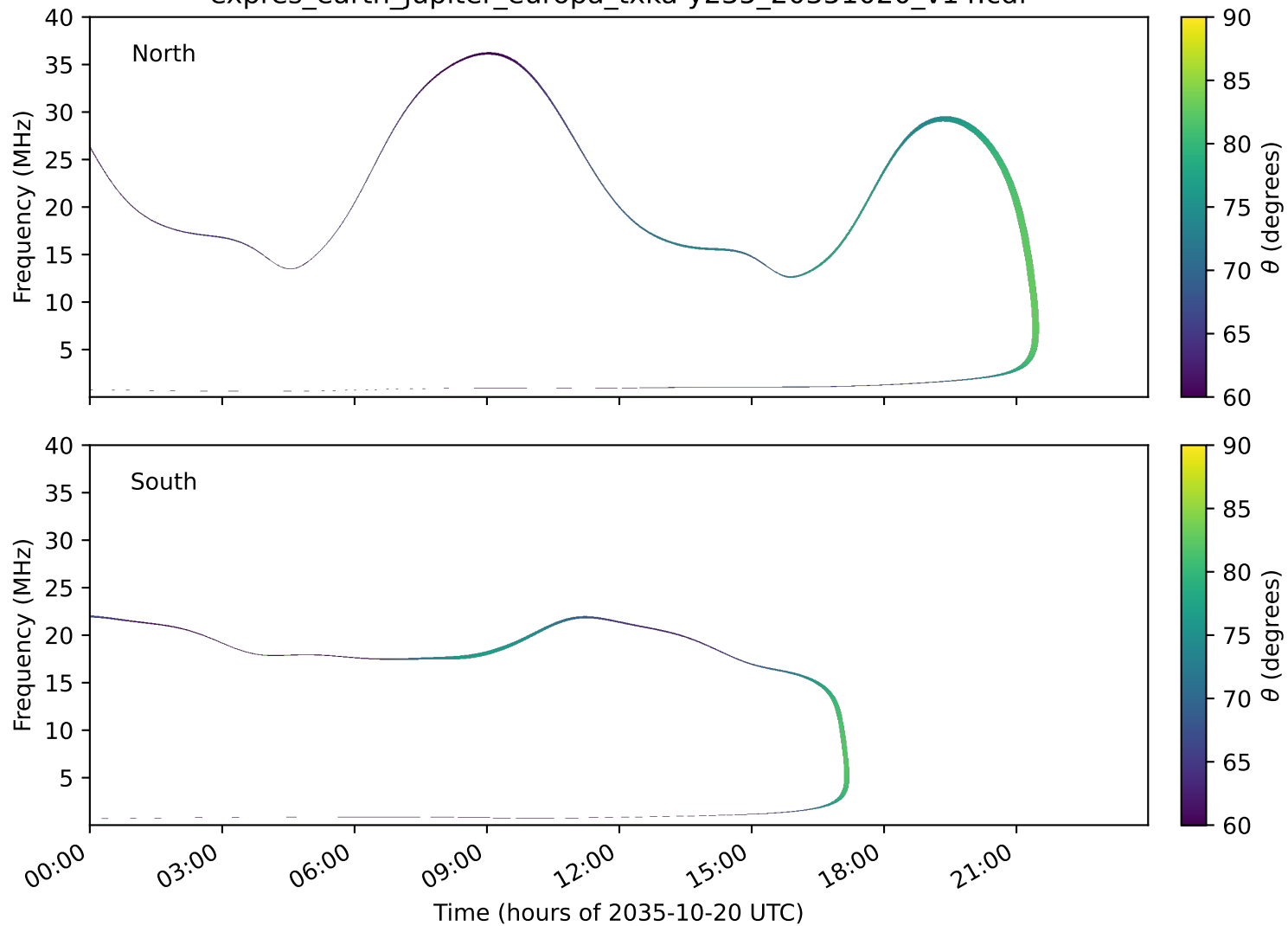
expres_earth_jupiter_europa_txka-y235_20351020_v14.cdf
