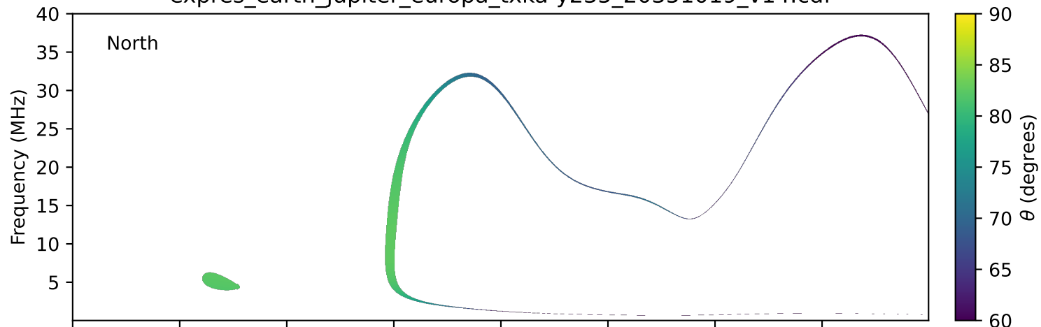
expres_earth_jupiter_europa_txka-y235_20351019_v14.cdf
