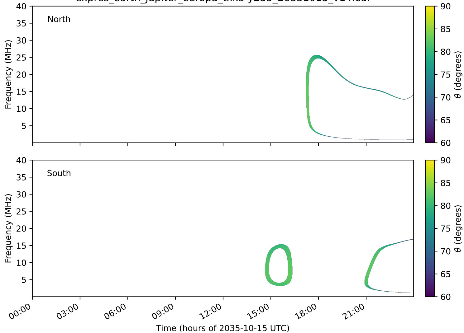
expres_earth_jupiter_europa_txka-y235_20351015_v14.cdf
