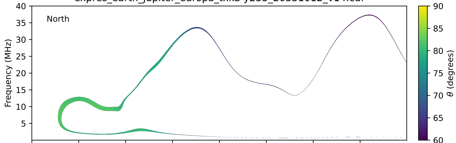
expres_earth_jupiter_europa_txka-y235_20351012_v14.cdf
