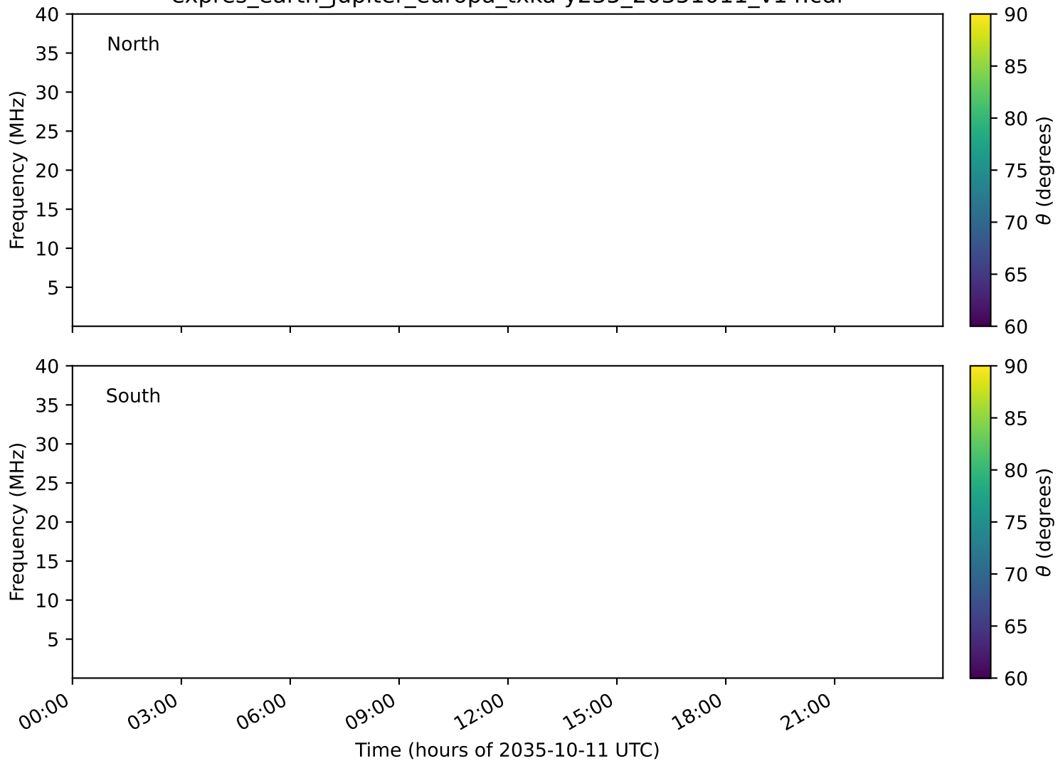
expres_earth_jupiter_europa_txka-y235_20351011_v14.cdf
