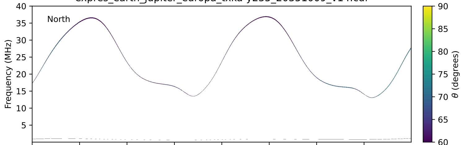
expres_earth_jupiter_europa_txka-y235_20351009_v14.cdf
