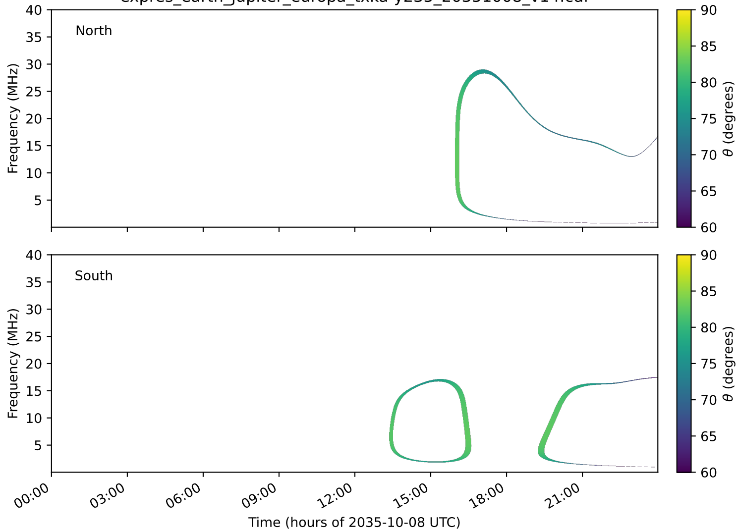
expres_earth_jupiter_europa_txka-y235_20351008_v14.cdf
