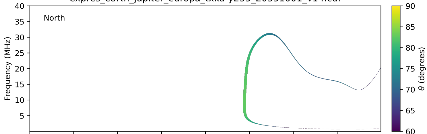
expres_earth_jupiter_europa_txka-y235_20351001_v14.cdf
