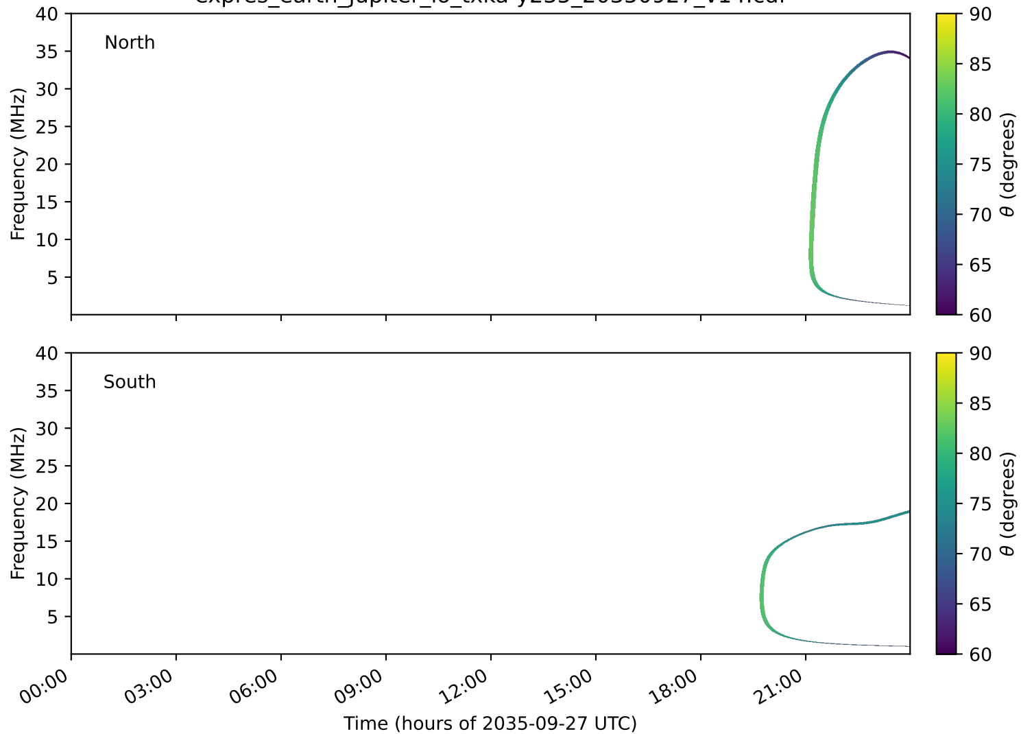
expres_earth_jupiter_io_txka-y235_20350927_v14.cdf
