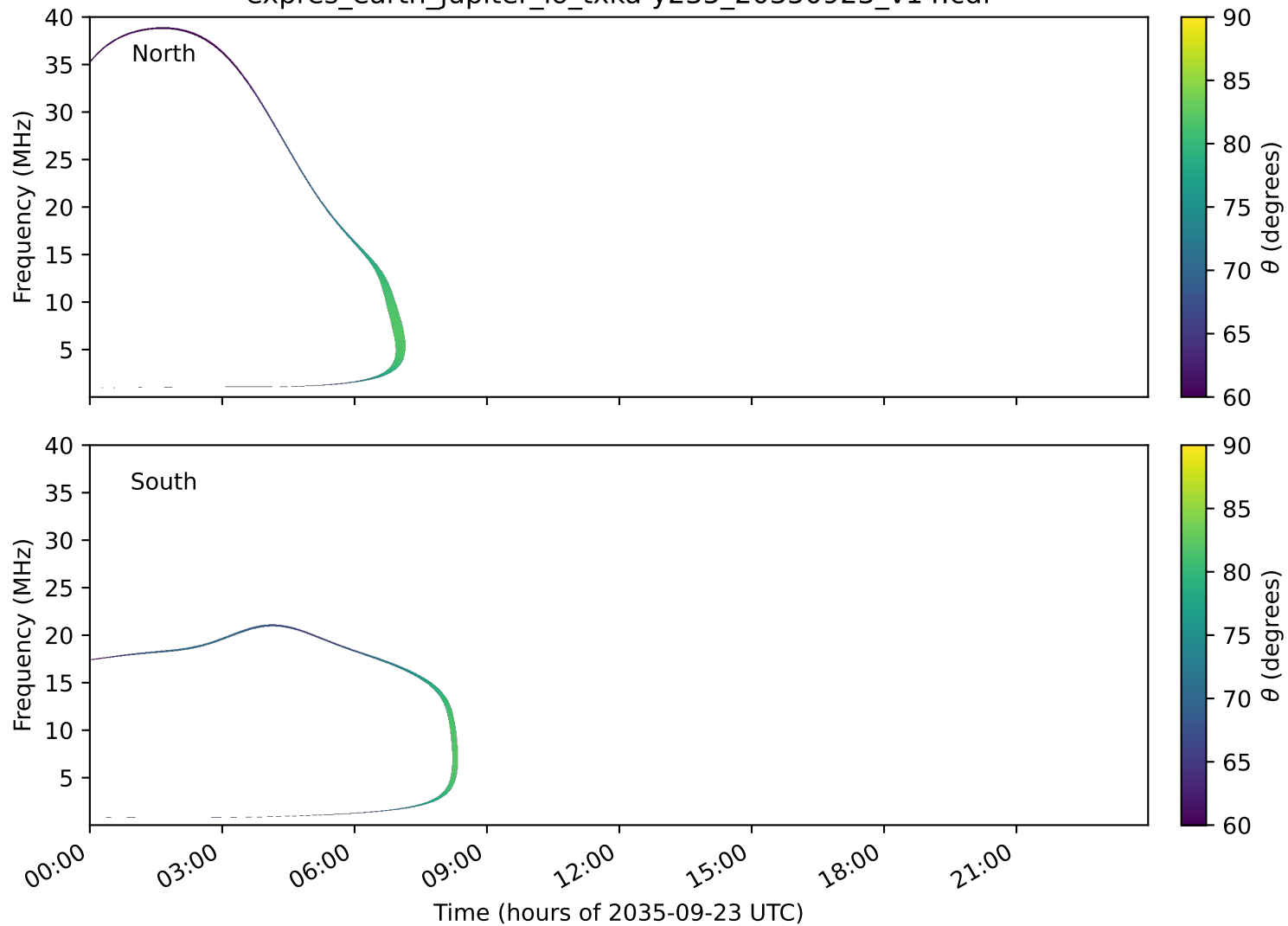
expres_earth_jupiter_io_txka-y235_20350923_v14.cdf
