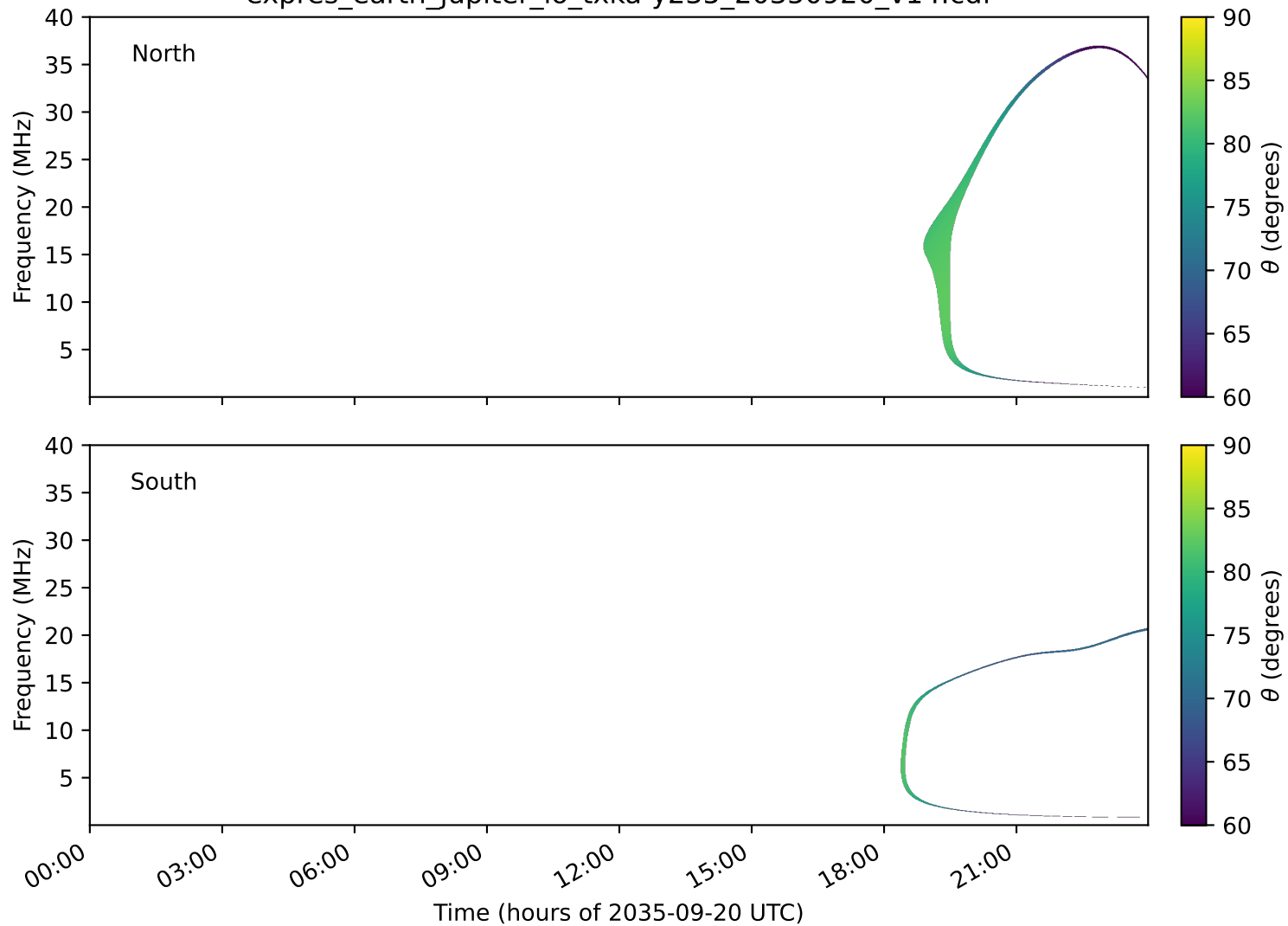
expres_earth_jupiter_io_txka-y235_20350920_v14.cdf
