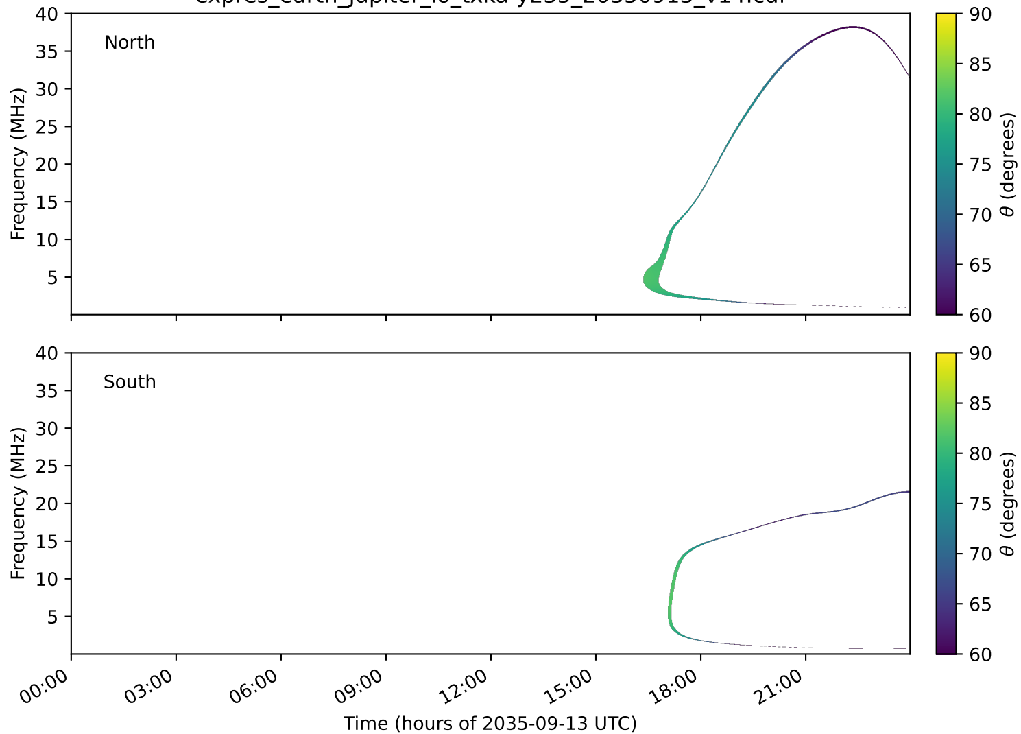
expres_earth_jupiter_io_txka-y235_20350913_v14.cdf
