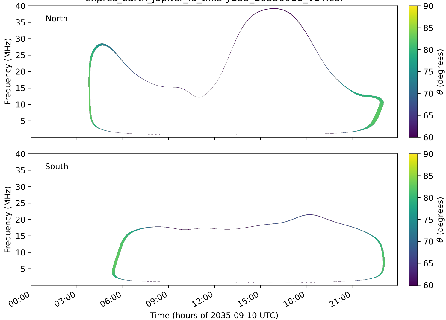
expres_earth_jupiter_io_txka-y235_20350910_v14.cdf
