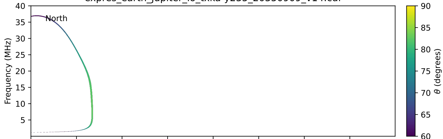
expres_earth_jupiter_io_txka-y235_20350909_v14.cdf
