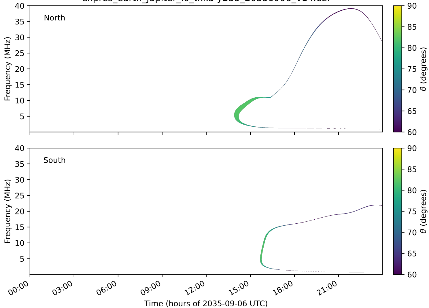
expres_earth_jupiter_io_txka-y235_20350906_v14.cdf
