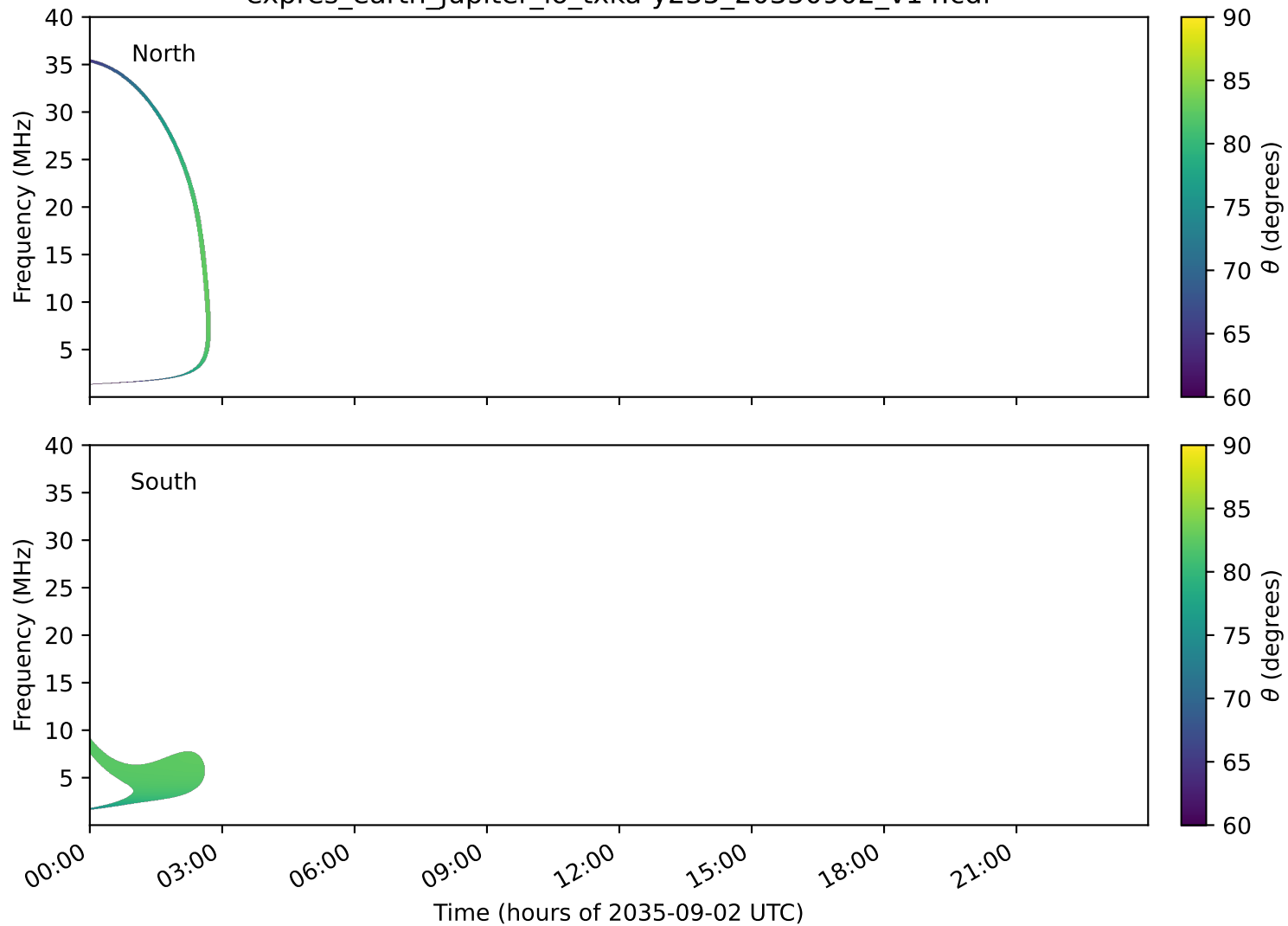
expres_earth_jupiter_io_txka-y235_20350902_v14.cdf
