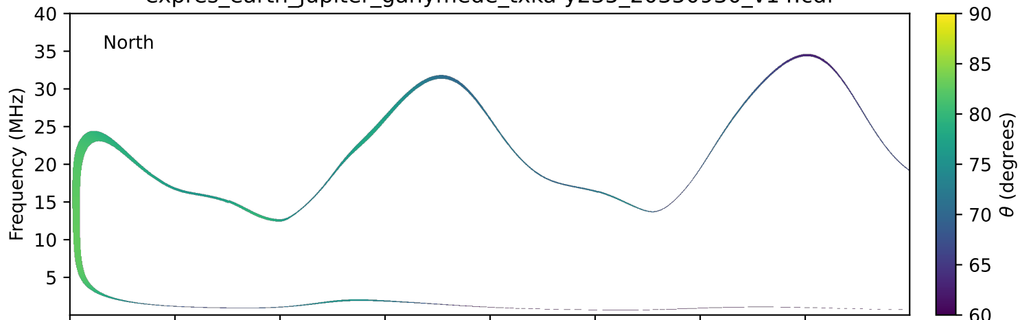
expres_earth_jupiter_ganymede_txka-y235_20350930_v14.cdf
