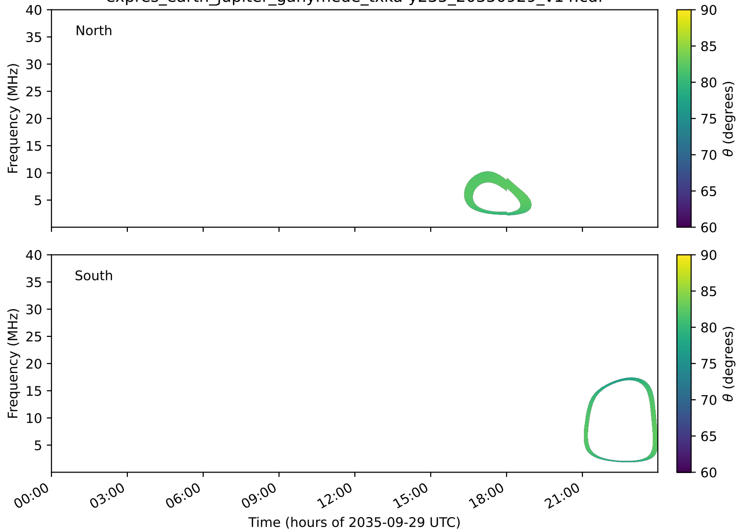
expres_earth_jupiter_ganymede_txka-y235_20350929_v14.cdf
