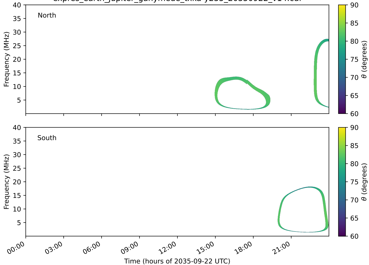
expres_earth_jupiter_ganymede_txka-y235_20350922_v14.cdf
