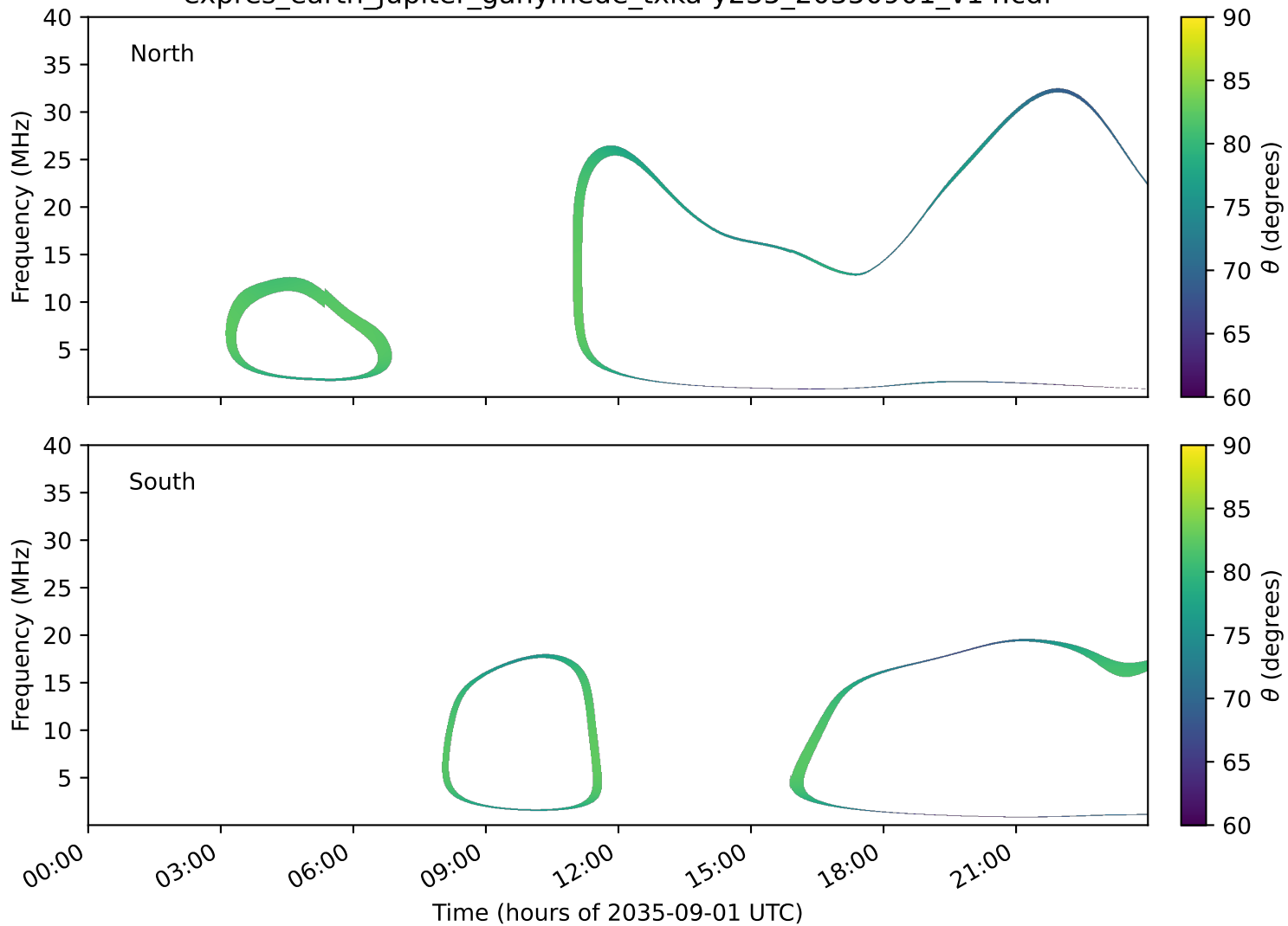
expres_earth_jupiter_ganymede_txka-y235_20350901_v14.cdf
