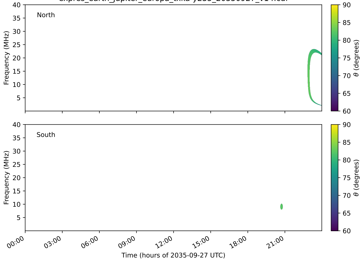
expres_earth_jupiter_europa_txka-y235_20350927_v14.cdf
