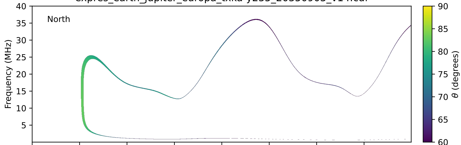
expres_earth_jupiter_europa_txka-y235_20350903_v14.cdf
