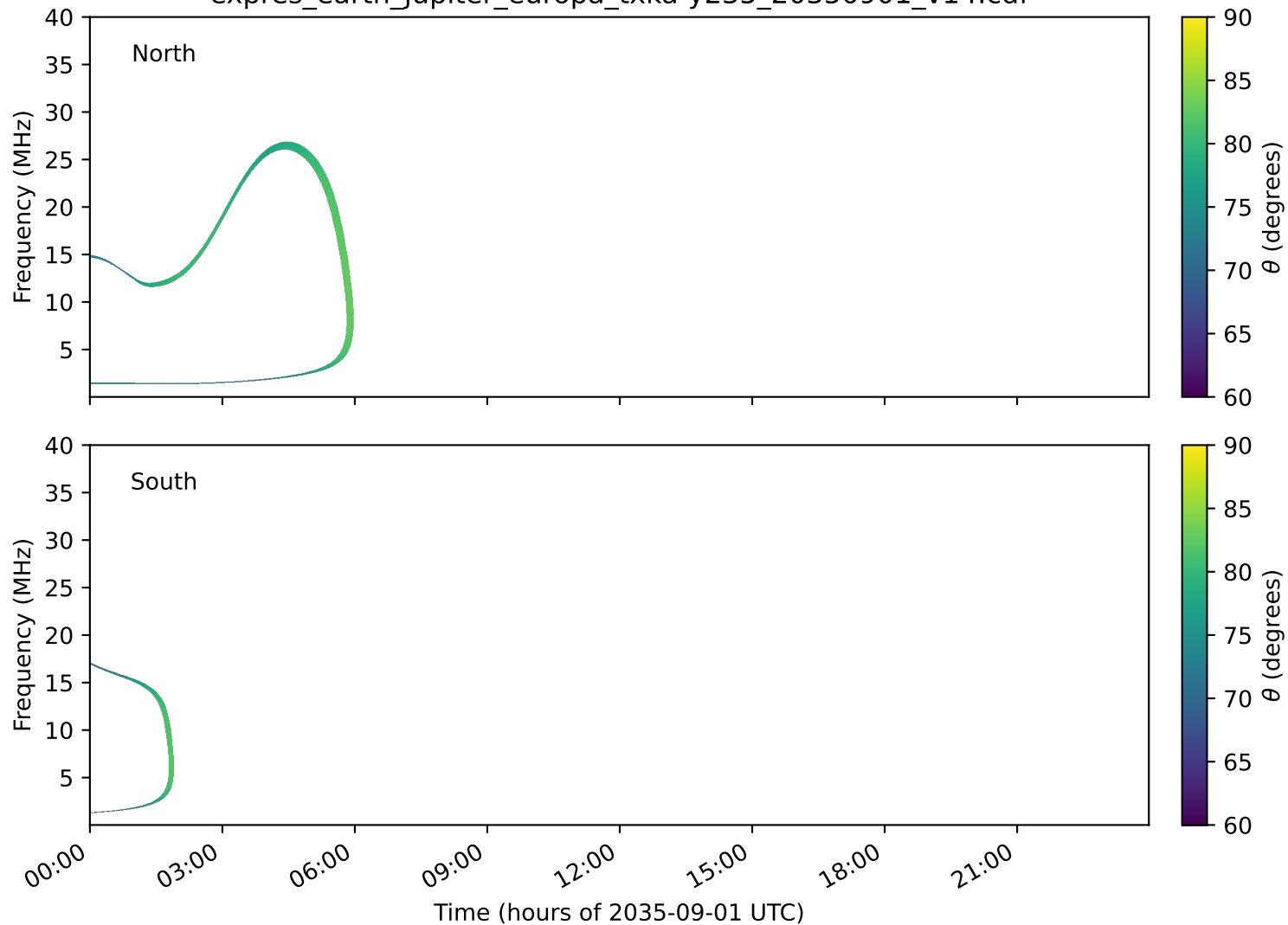
expres_earth_jupiter_europa_txka-y235_20350901_v14.cdf
