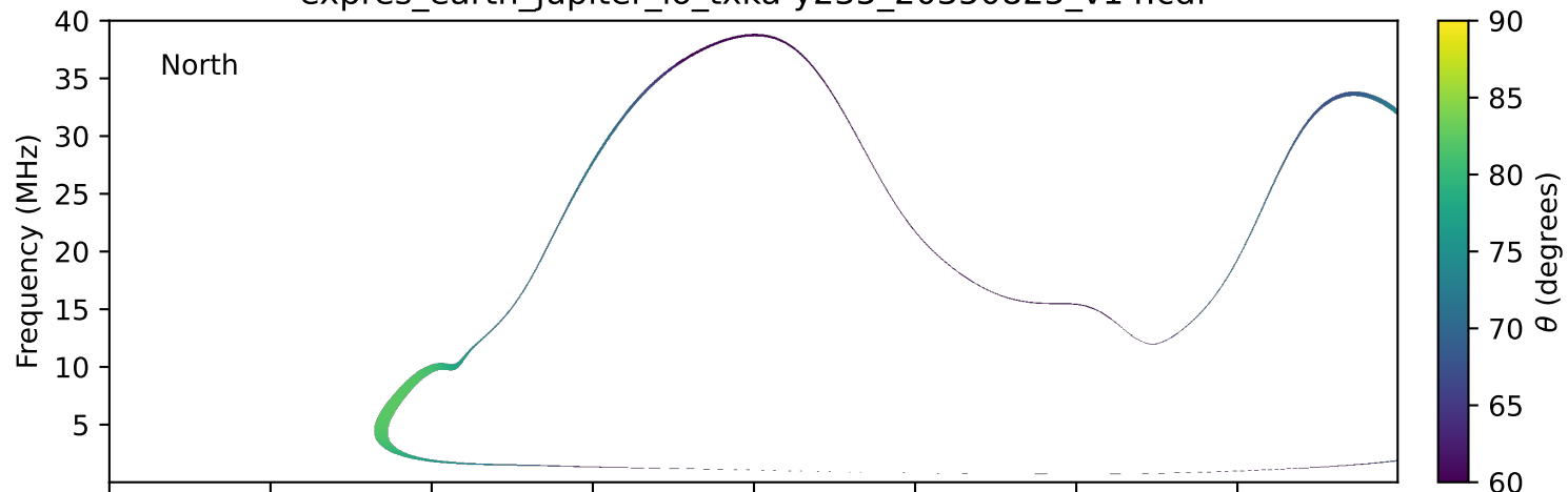
expres_earth_jupiter_io_txka-y235_20350825_v14.cdf
