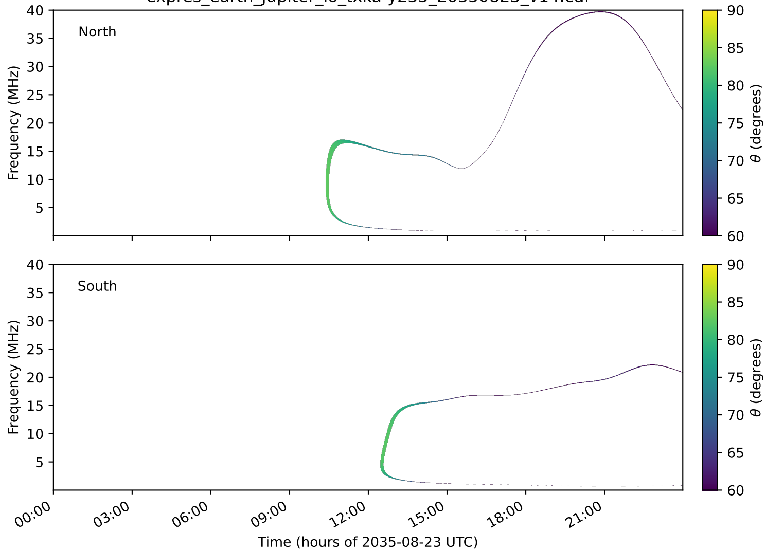
expres_earth_jupiter_io_txka-y235_20350823_v14.cdf
