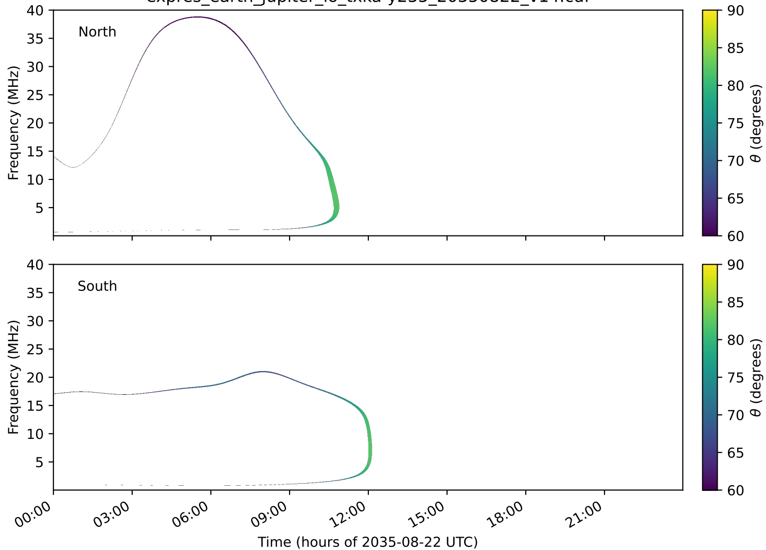
expres_earth_jupiter_io_txka-y235_20350822_v14.cdf
