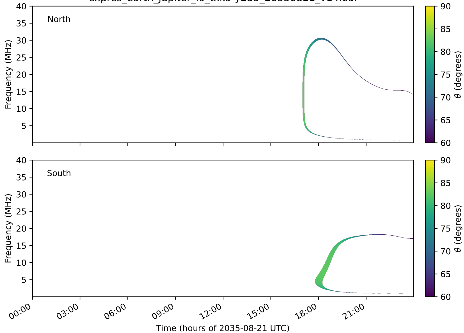
expres_earth_jupiter_io_txka-y235_20350821_v14.cdf
