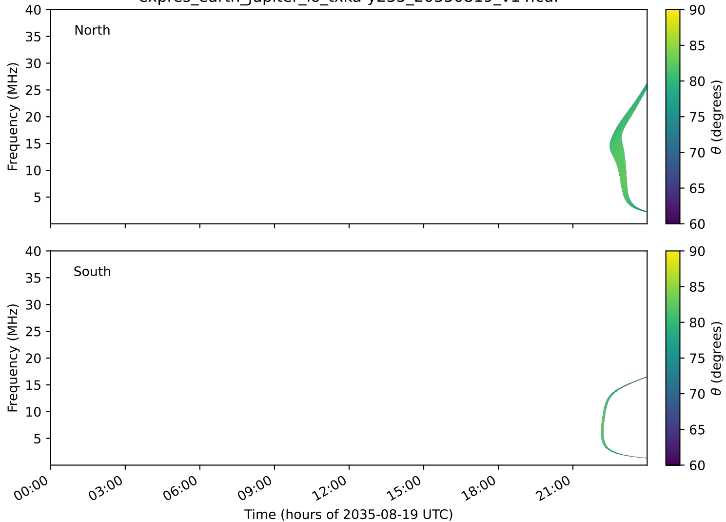
expres_earth_jupiter_io_txka-y235_20350819_v14.cdf
