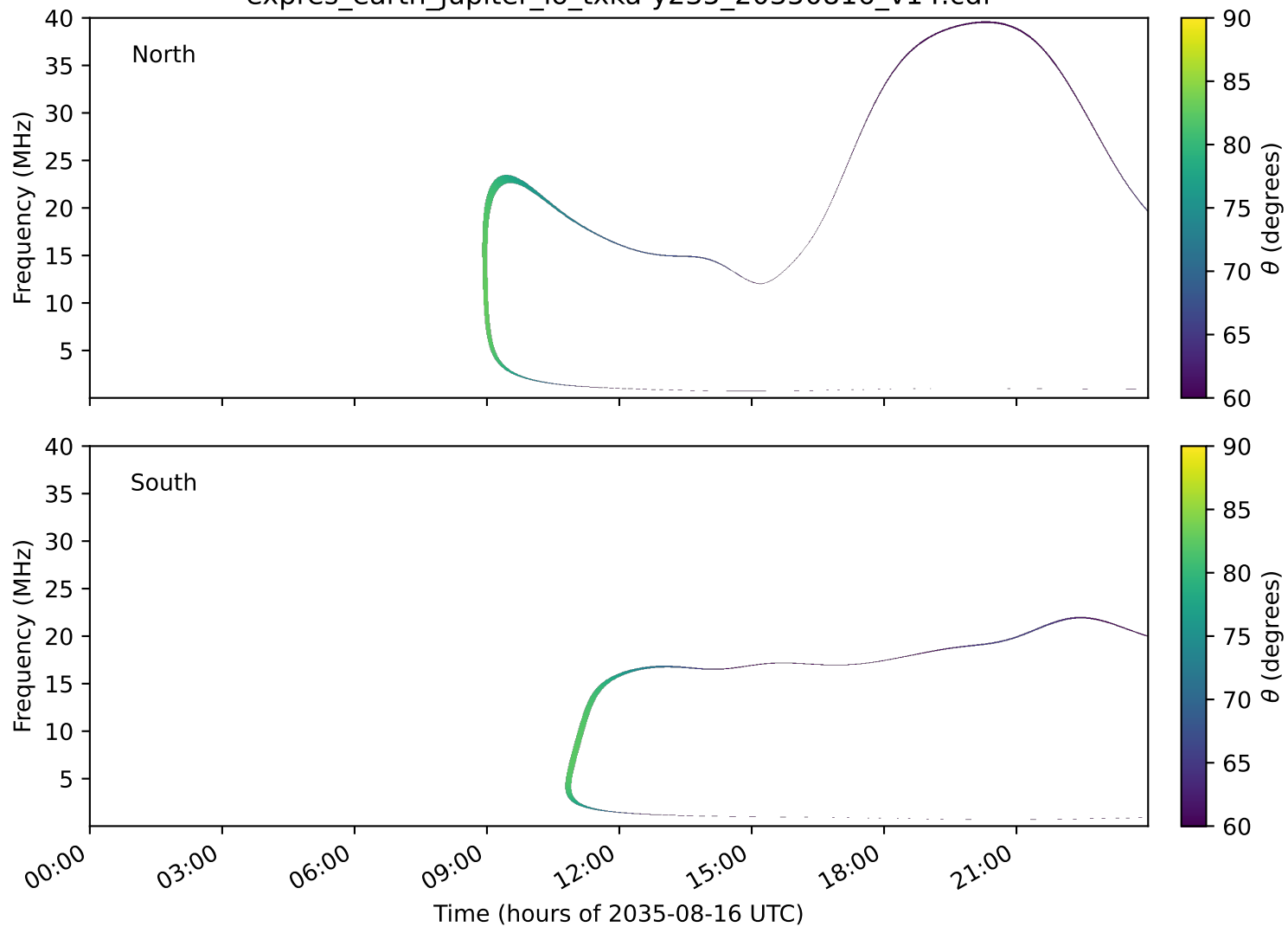
expres_earth_jupiter_io_txka-y235_20350816_v14.cdf
