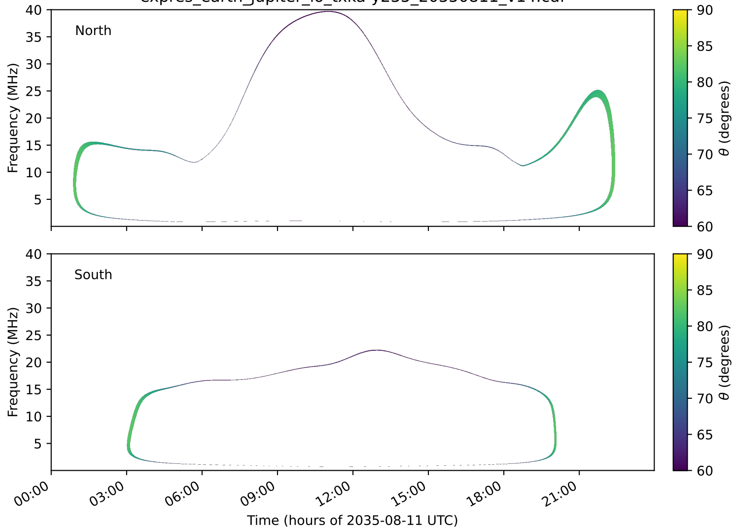
expres_earth_jupiter_io_txka-y235_20350811_v14.cdf
