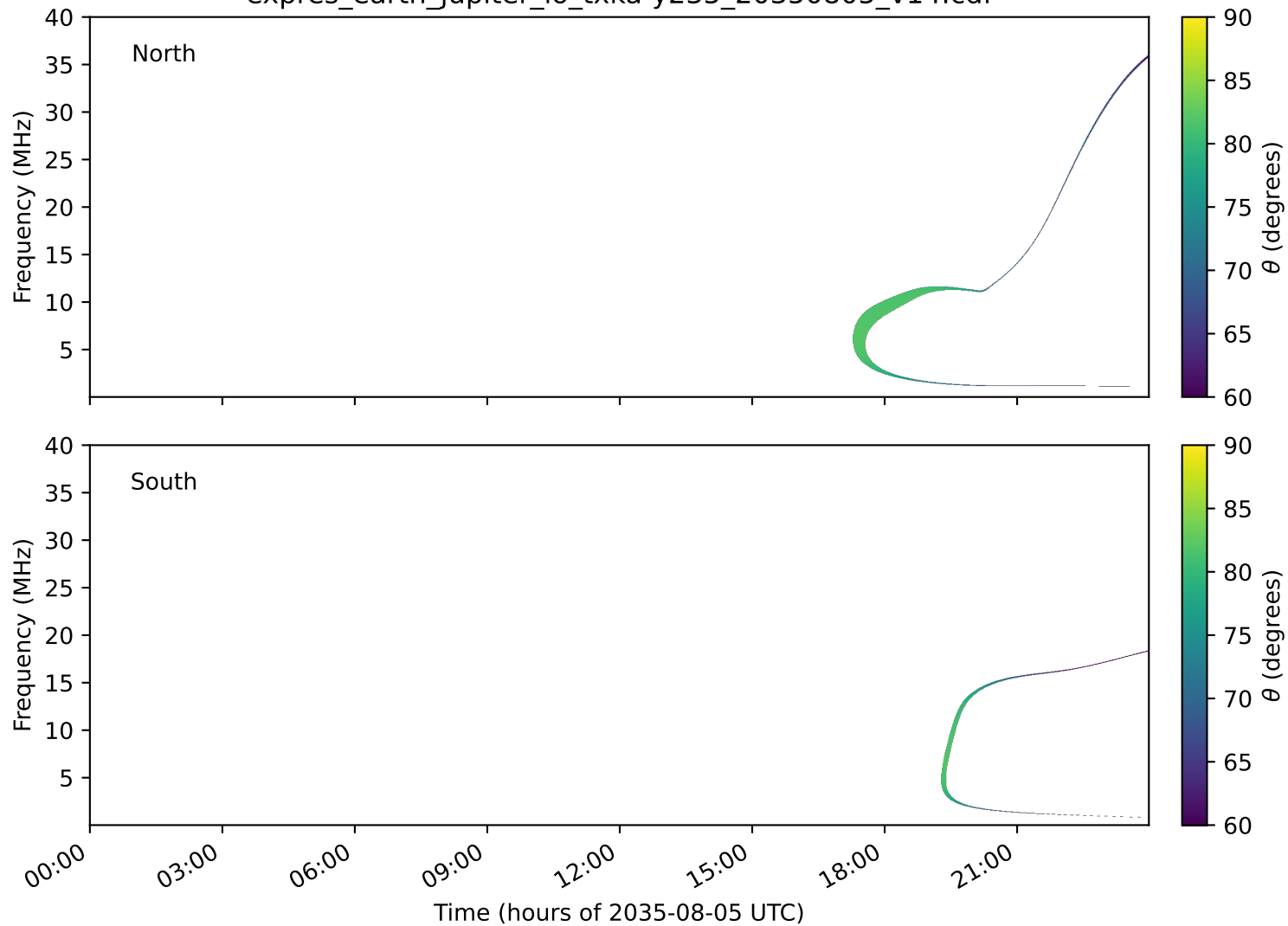
expres_earth_jupiter_io_txka-y235_20350805_v14.cdf
