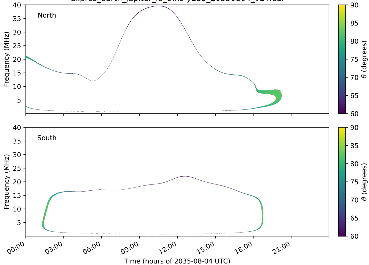
expres_earth_jupiter_io_txka-y235_20350804_v14.cdf
