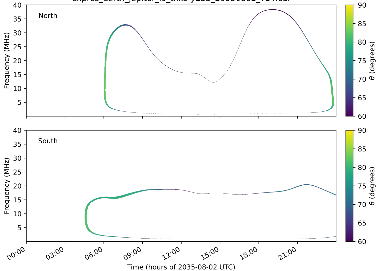
expres_earth_jupiter_io_txka-y235_20350802_v14.cdf
