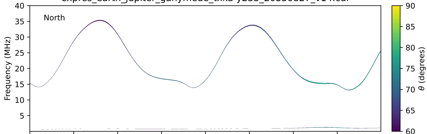
expres_earth_jupiter_ganymede_txka-y235_20350827_v14.cdf
