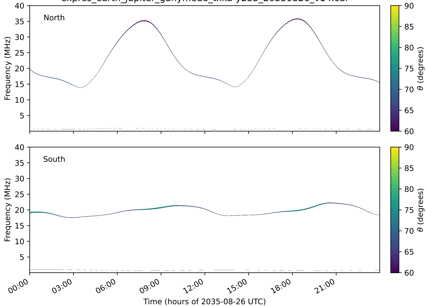
expres_earth_jupiter_ganymede_txka-y235_20350826_v14.cdf
