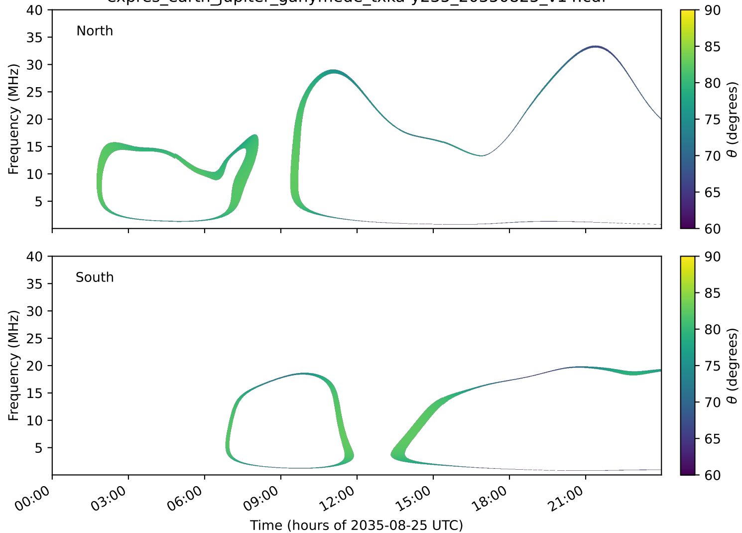
expres_earth_jupiter_ganymede_txka-y235_20350825_v14.cdf
