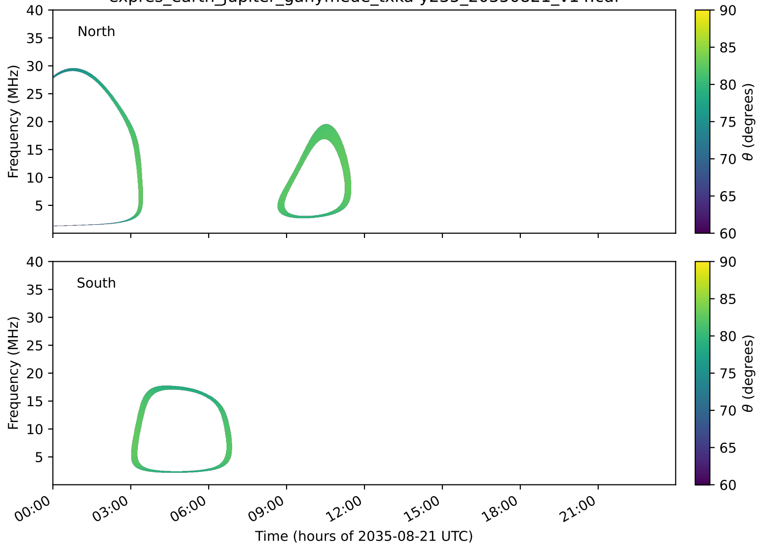
expres_earth_jupiter_ganymede_txka-y235_20350821_v14.cdf
