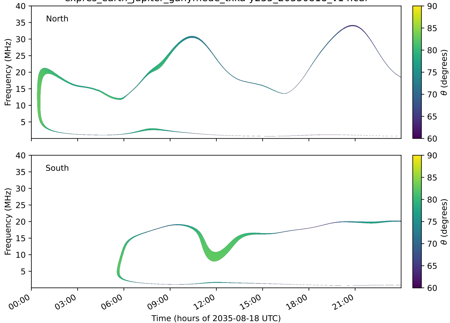
expres_earth_jupiter_ganymede_txka-y235_20350818_v14.cdf
