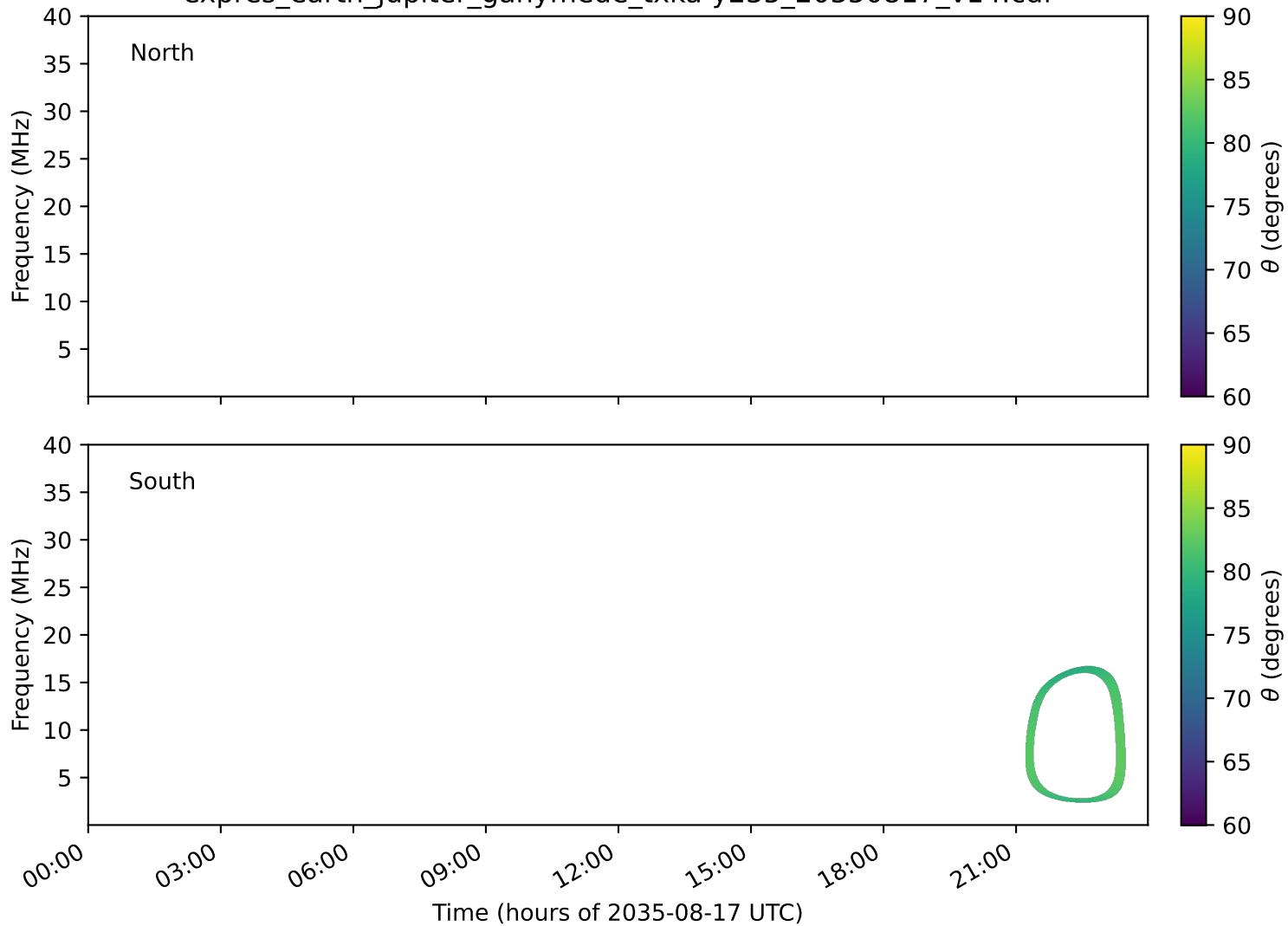
expres_earth_jupiter_ganymede_txka-y235_20350817_v14.cdf
