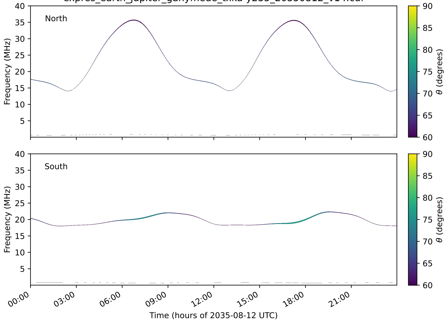
expres_earth_jupiter_ganymede_txka-y235_20350812_v14.cdf
