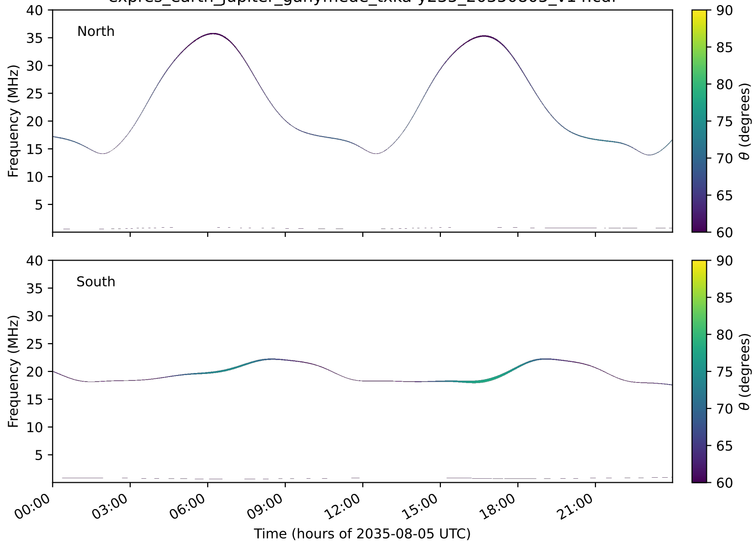
expres_earth_jupiter_ganymede_txka-y235_20350805_v14.cdf
