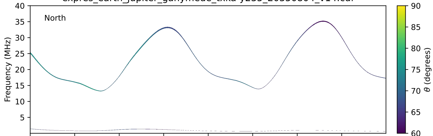
expres_earth_jupiter_ganymede_txka-y235_20350804_v14.cdf
