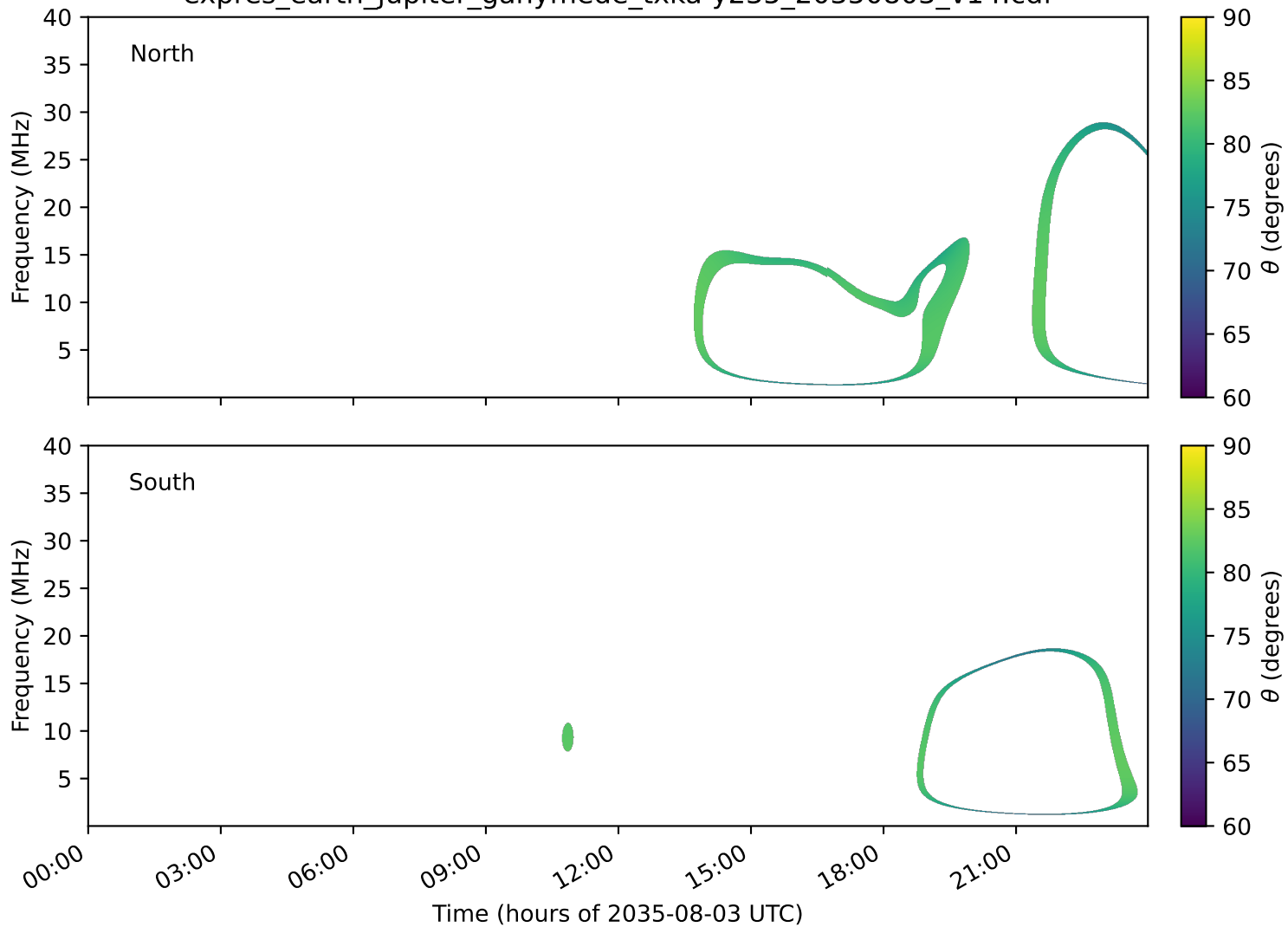
expres_earth_jupiter_ganymede_txka-y235_20350803_v14.cdf
