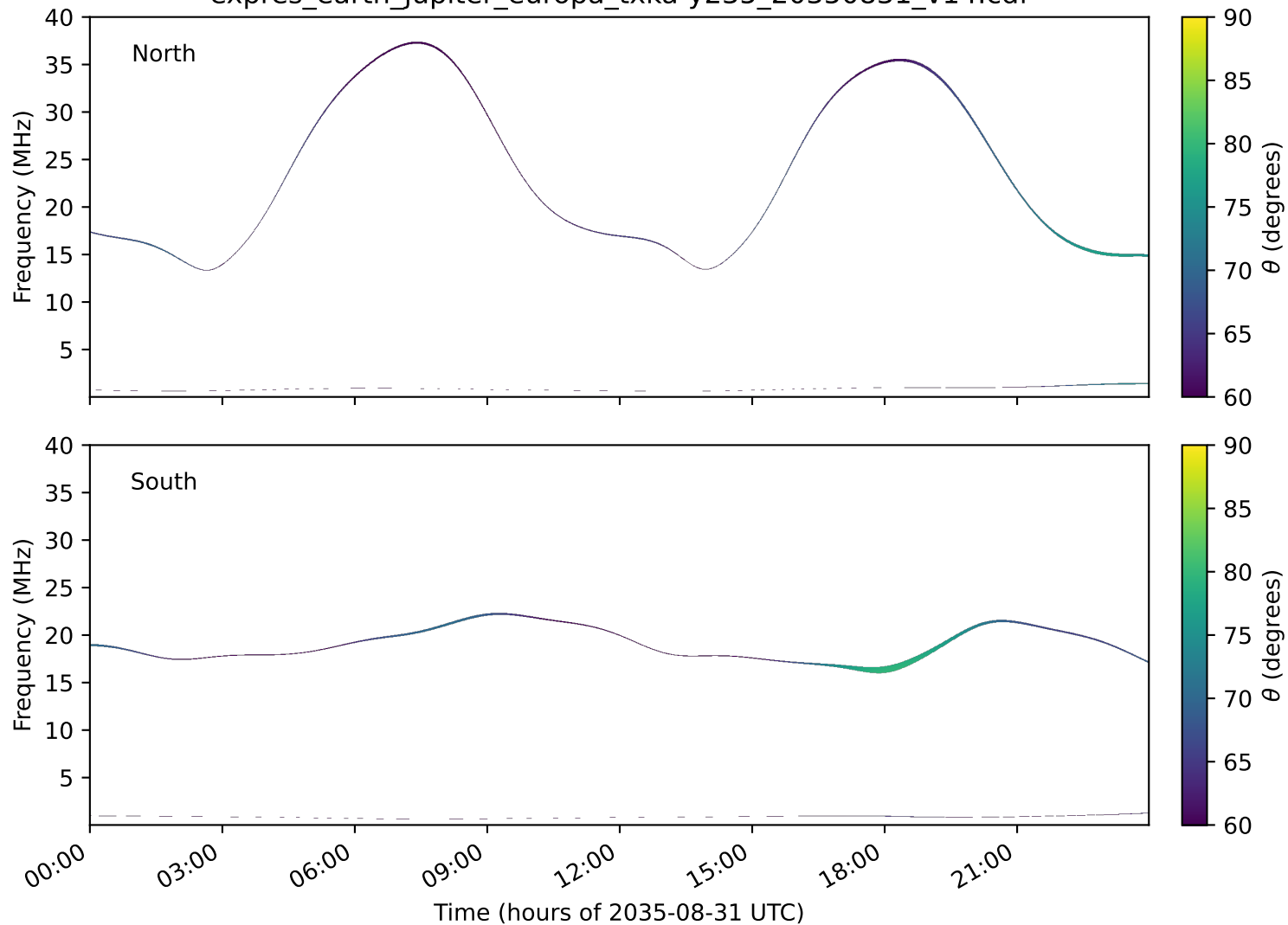
expres_earth_jupiter_europa_txka-y235_20350831_v14.cdf
