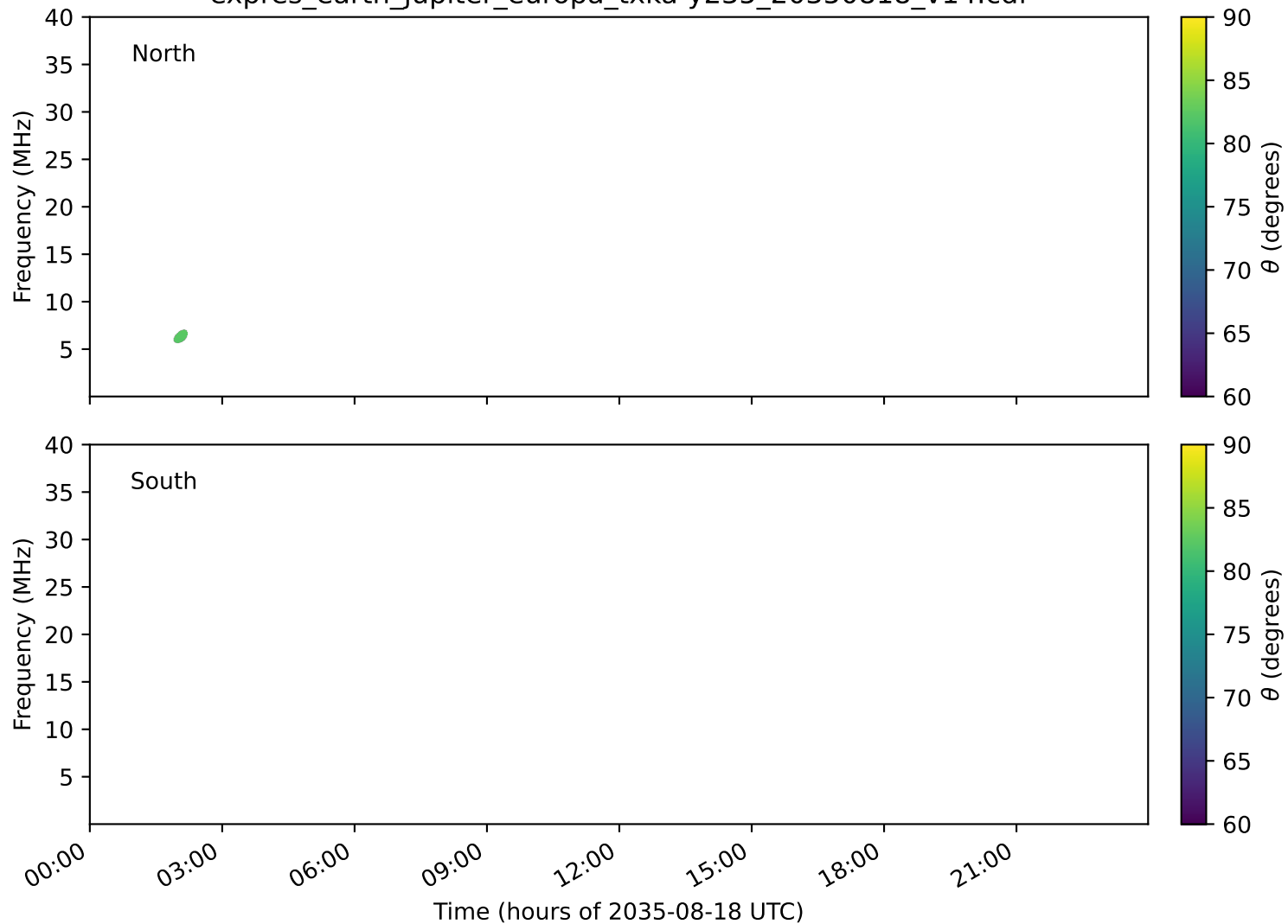
expres_earth_jupiter_europa_txka-y235_20350818_v14.cdf
