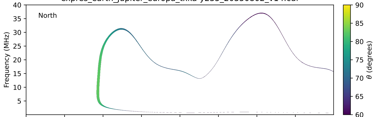
expres_earth_jupiter_europa_txka-y235_20350802_v14.cdf
