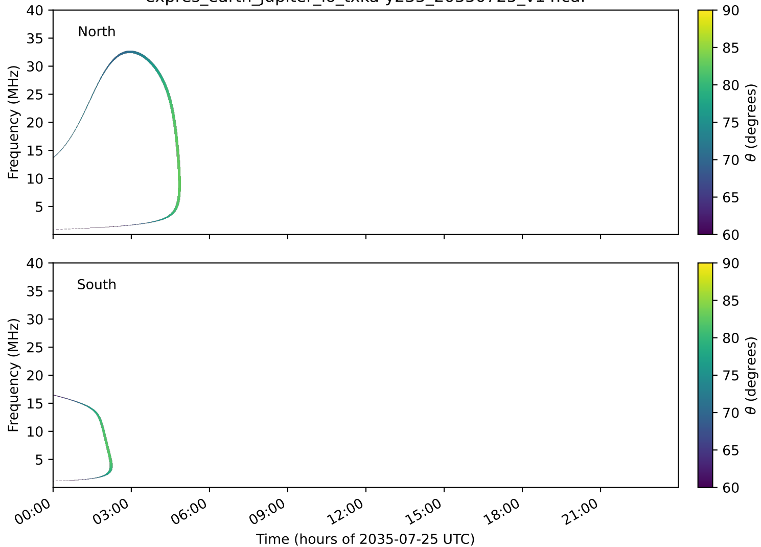
expres_earth_jupiter_io_txka-y235_20350725_v14.cdf
